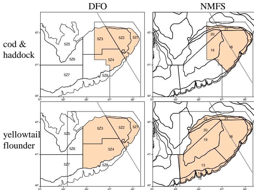
Figure 2. DFO and NMFS survey strata used to develop biomass indices on either side of the Canada/USA boundary for Eastern Georges Bank cod and haddock and Georges Bank yellowtail flounder in relation to the management unit borders. Strata boundaries (thin black lines) with strata labels are shown. The shaded area represents the strata and strata sections that were used to approximate the respective management units (thick grey lines).
