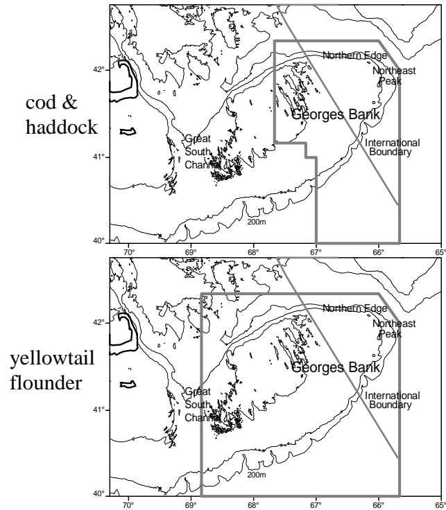
Figure 1. The management areas for cod and haddock (upper panel) and yellowtail flounder (lower panel) on Georges Bank and the Canada/USA boundary line across which resource distribution was determined.
